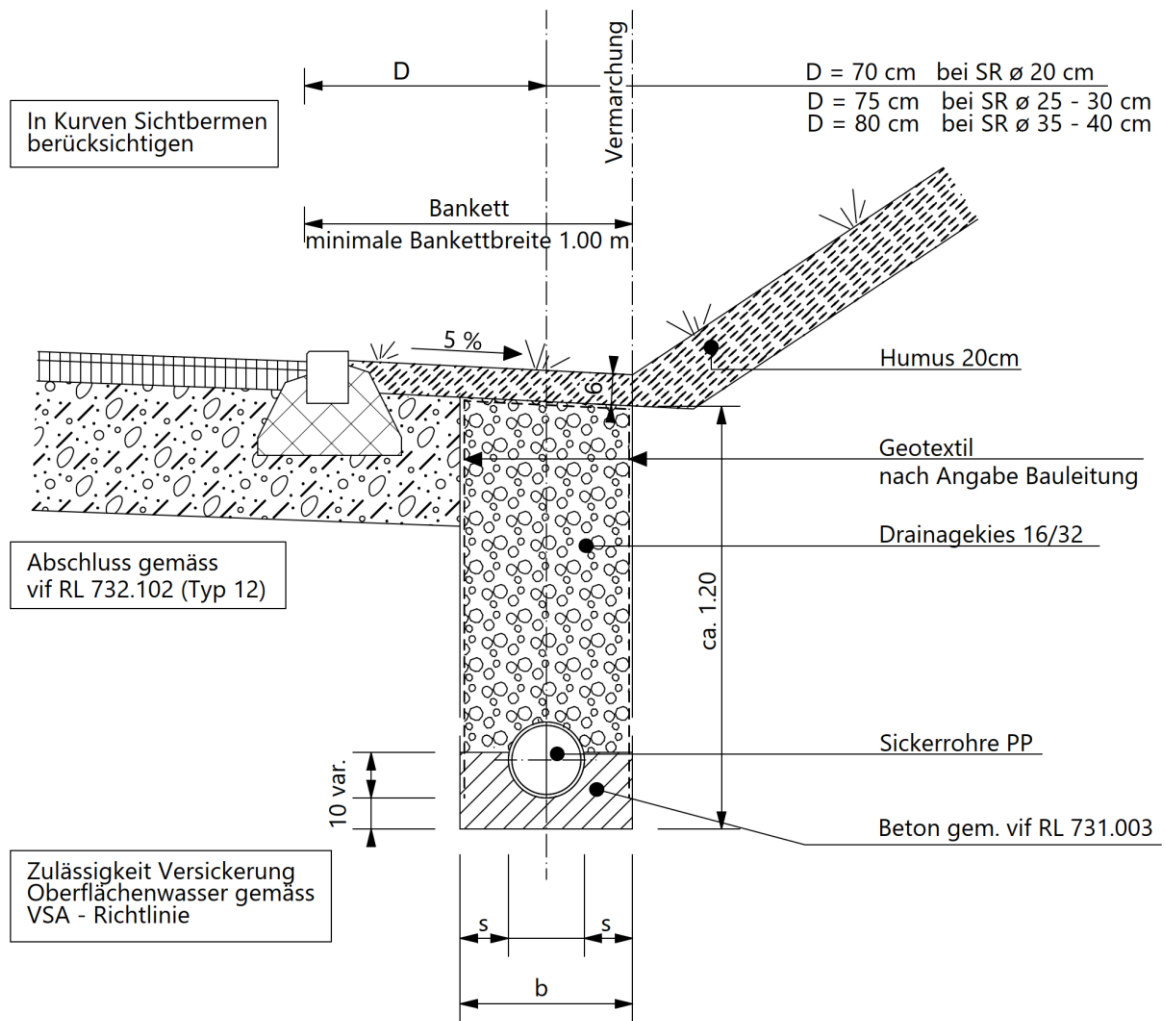
PP - Sickerrohre
